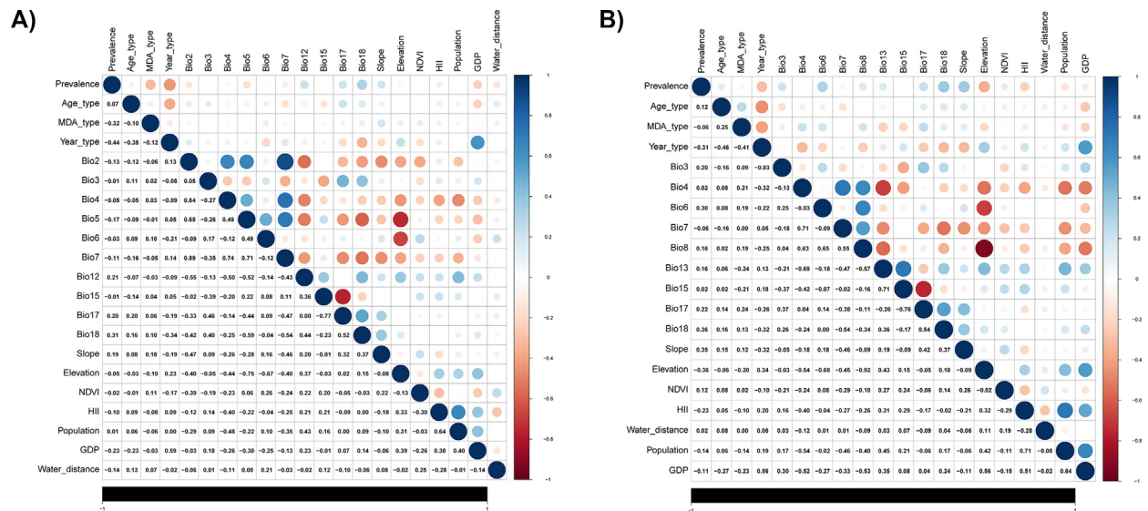
Fig. 2. Correlation matrix of the relationship between variables in S. haematobium and S. mansoni
